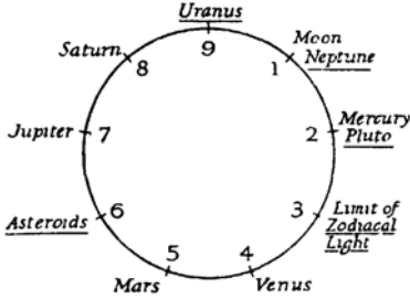
Fig 6 The Octave of the Planets (Underlined • Invisible)
