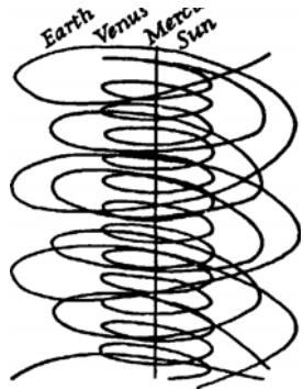
(b) Part of the Solar System, in Time
