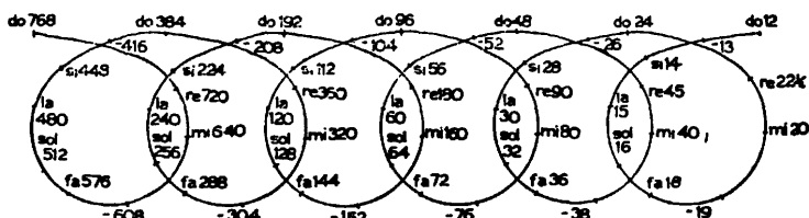
Fig. 10: The Octaves of Molecular Compounds See Appendix
